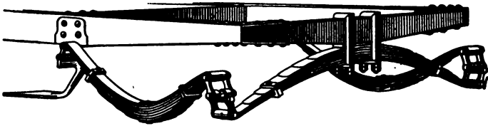
FIG. 82.—Three-point suspended spring, or platform spring, one of the latest and most conspicuous improvements in spring suspension designs.
